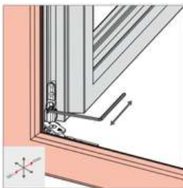
Lateral adjustment Min.: -1.5mm Max.: +2.0mm
