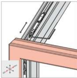
Lateral adjustment Min.: -2.0mm Max.: +2.0mm
