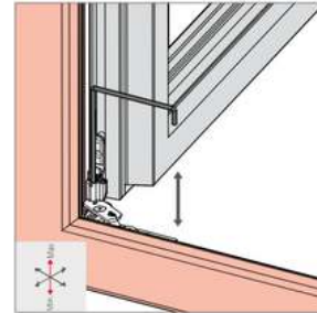
Height adjustment Min.: -1.0mm Max.: +2.0
